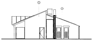
East Elevation
